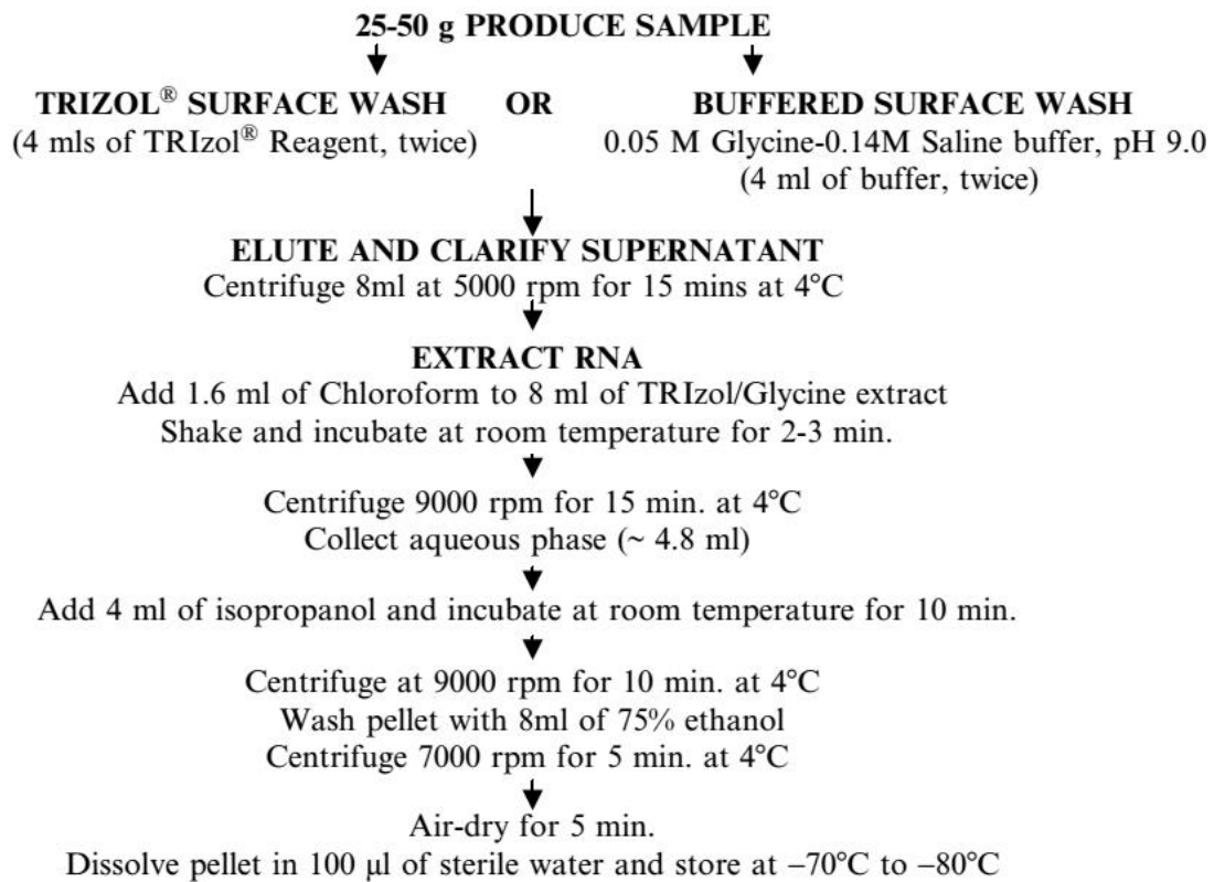
Figure Virus concentration and extraction from produce using TRIZOL ® or glycine-saline buffer (modifications of protocol by Schwab et al. (91)).
